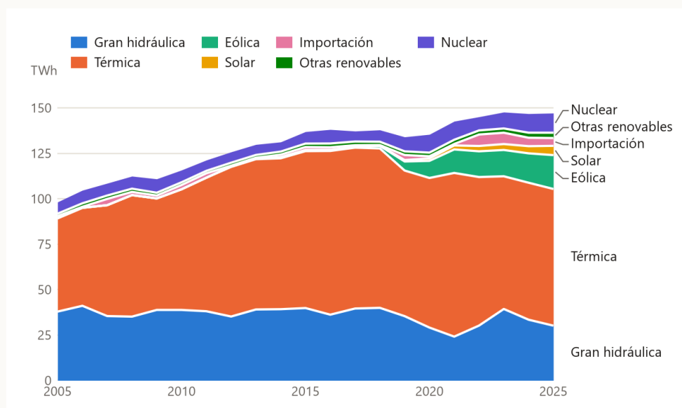
Electricity generation by source, 2005–2025, in TWh. Source: CAMMESA, annual statistics 5 .
