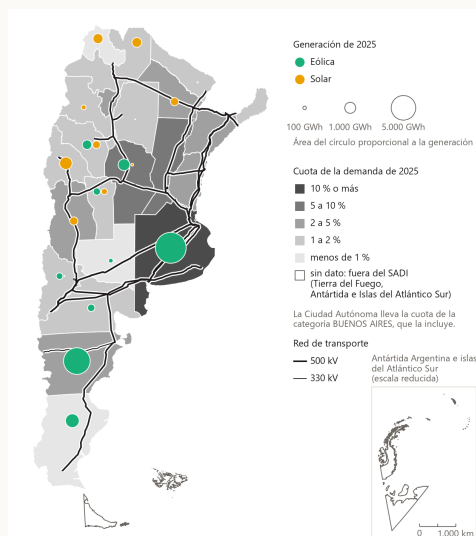
Figure. The 500 kV transmission grid and wind and solar plants, with 2025 demand by CAMMESA territorial category ■ 33 .
